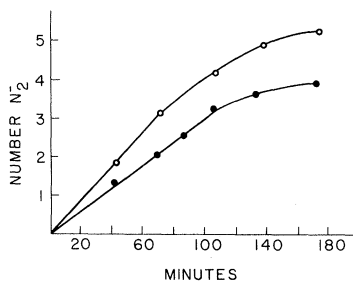
FIG. 3. Plot of the growth of the N_2^- for the two different polarizations of the damage producing uv light. The top curve is obtained for the \vec{E} vector parallel to [001] of the lattice. The lesser growth is obtained when the \vec{E} vector is parallel to the [100] direction.
