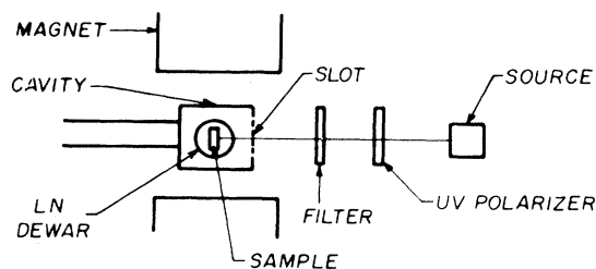
FIG. 1. Experimental arrangement for measuring the growth of the ESR signal of the \text{N}_2^- while simultaneously irradiating with uv light.
