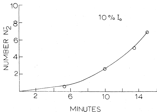
FIG. 4. A plot of the growth of the N_2^- versus time showing more detail in the early region of the curve. The numbers on the vertical axis of Figs. 3 and 4 are arbitrary and bear no relationship to each other as different uv sources were used in both sets of data.
