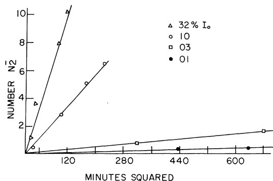
FIG. 5. A plot of the number of N_2^- versus the square of the time for different relative intensities of the damage producing light. The experiment was performed by placing neutral density filters between the source and the crystal. The I_0 refers to the intensity of the unfiltered light.
