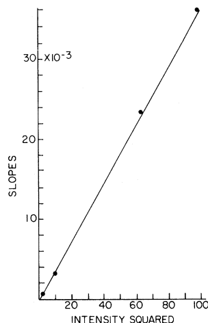
FIG. 6. Plot of the slopes of the lines of Fig. 5 versus the square of the relative intensity of the ultraviolet light.
