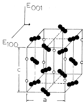
FIG. 2. The unit cell of potassium azide. The two orientations of the \vec{E} vector of the polarized light that were used to measure the growth of the N_2^- are shown.
